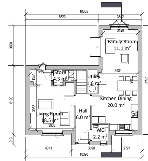
③ Type 3 Terraced Level 00 (Extended) 1 : 200
