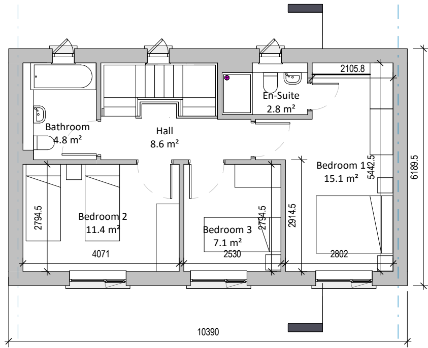
② Type 3 Terraced Level 01 1 : 100
