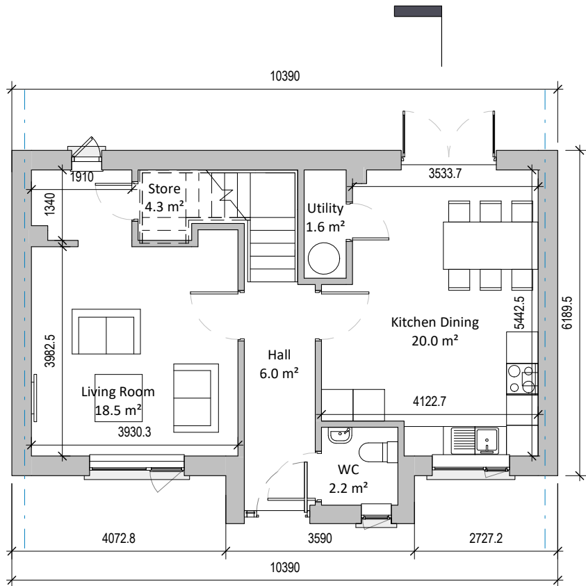
① Type 3 Terraced Level 00 1 : 100
